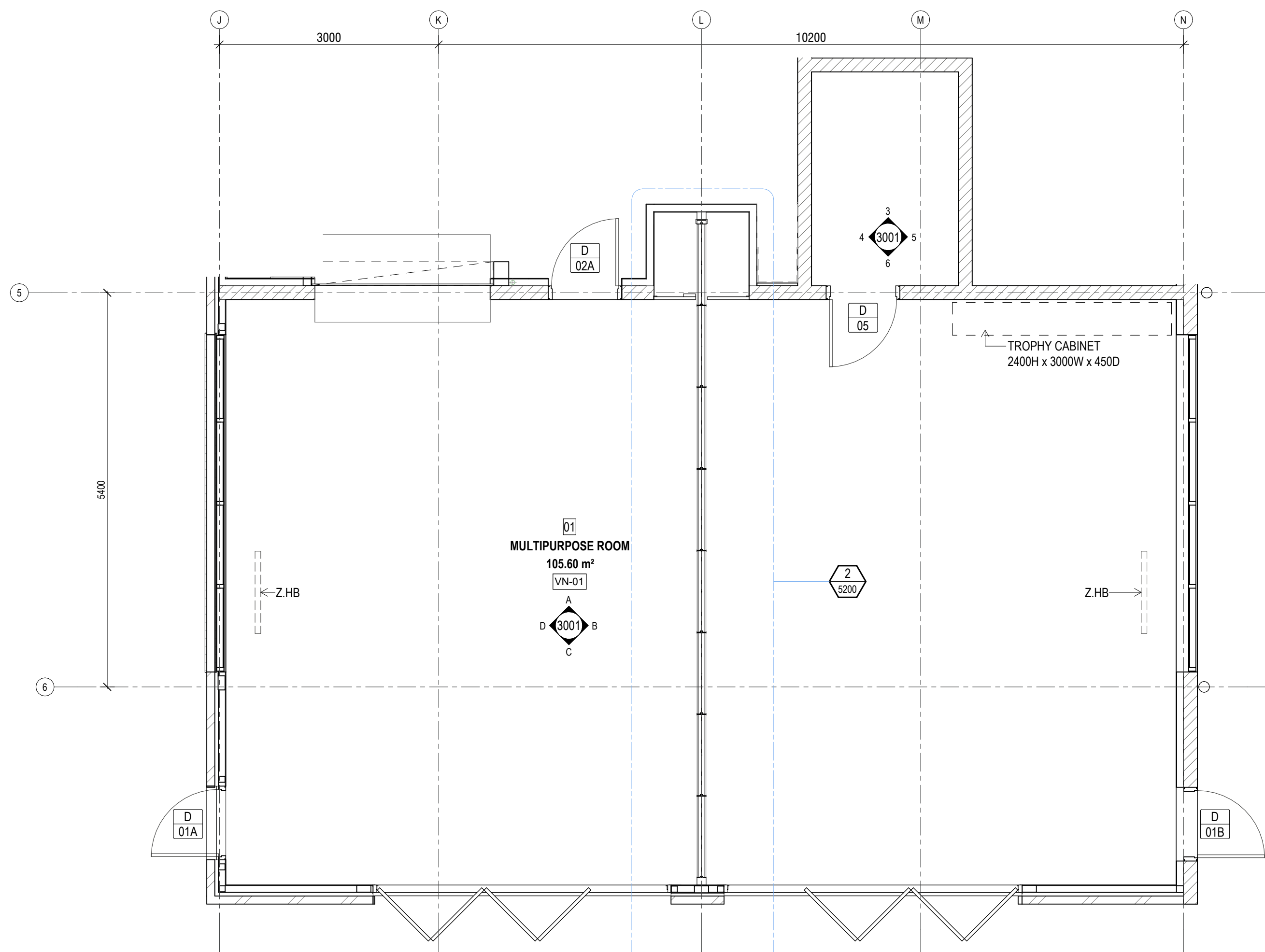
1 PLAN MULTI-PURPOSE ROOM Scale: 1 : 50
