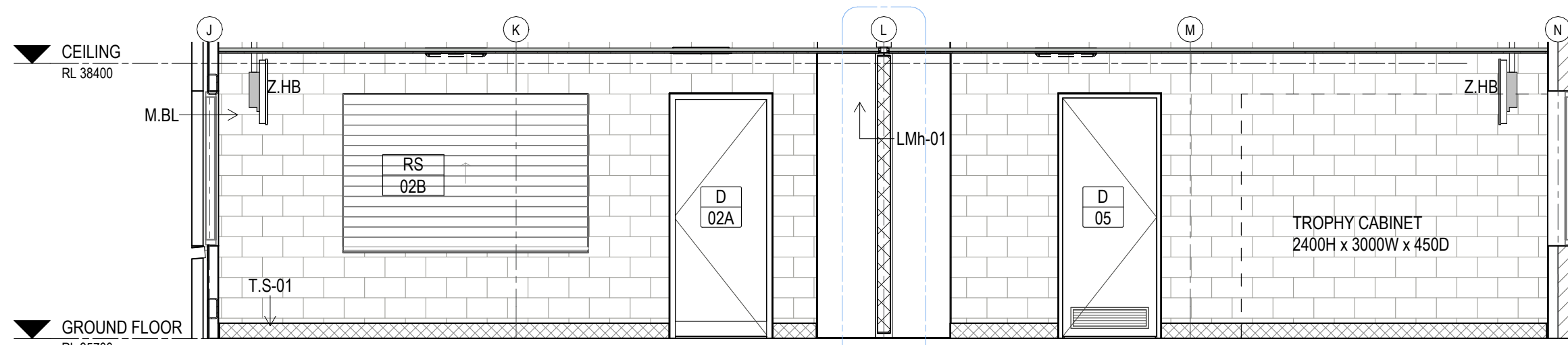
A ELEVATION MULTI-PURPOSE ROOM Scale: 1 : 50
