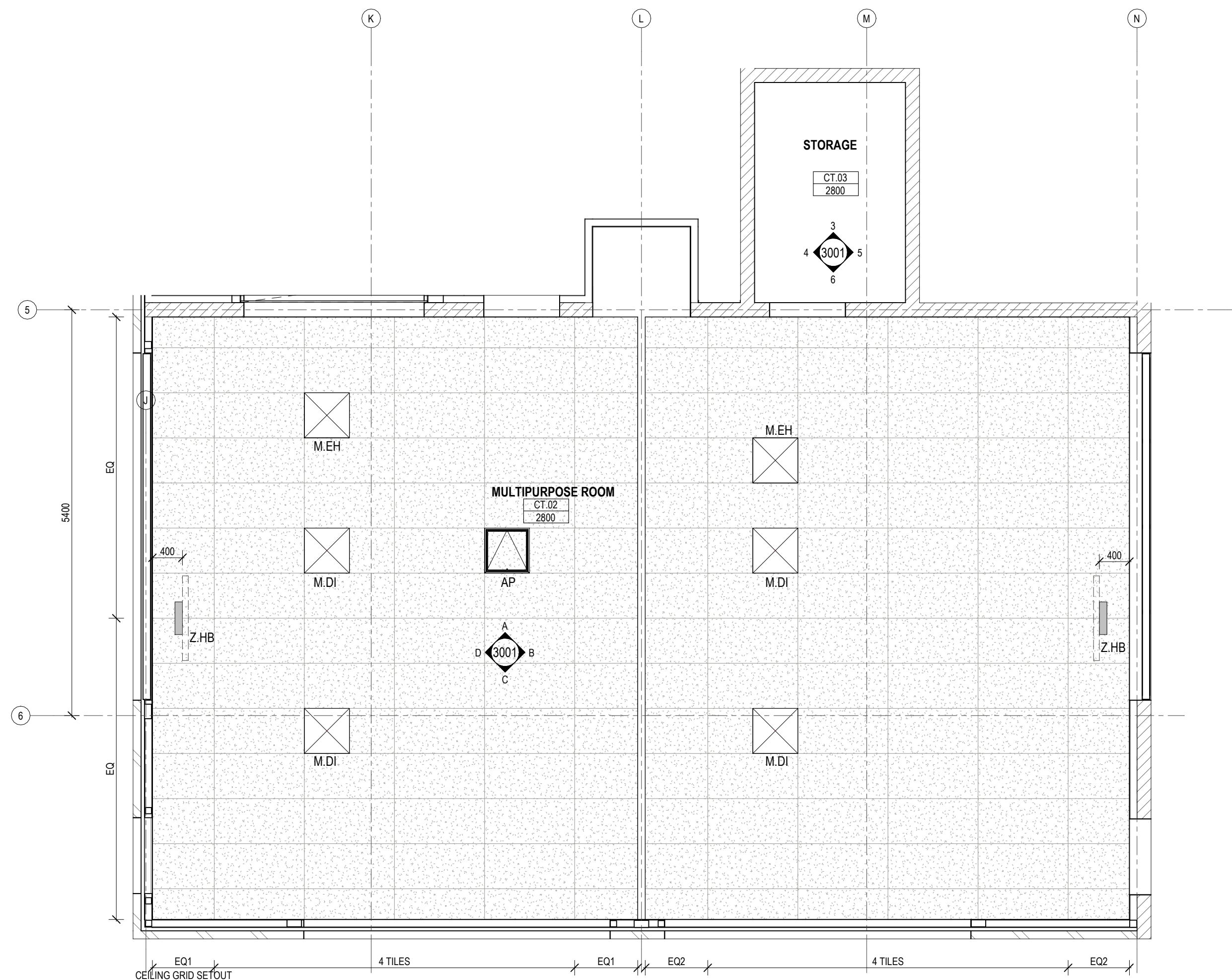
2 REFLECTED CEILING PLAN MULTI-PURPOSE ROOM Scale: 1 : 50
