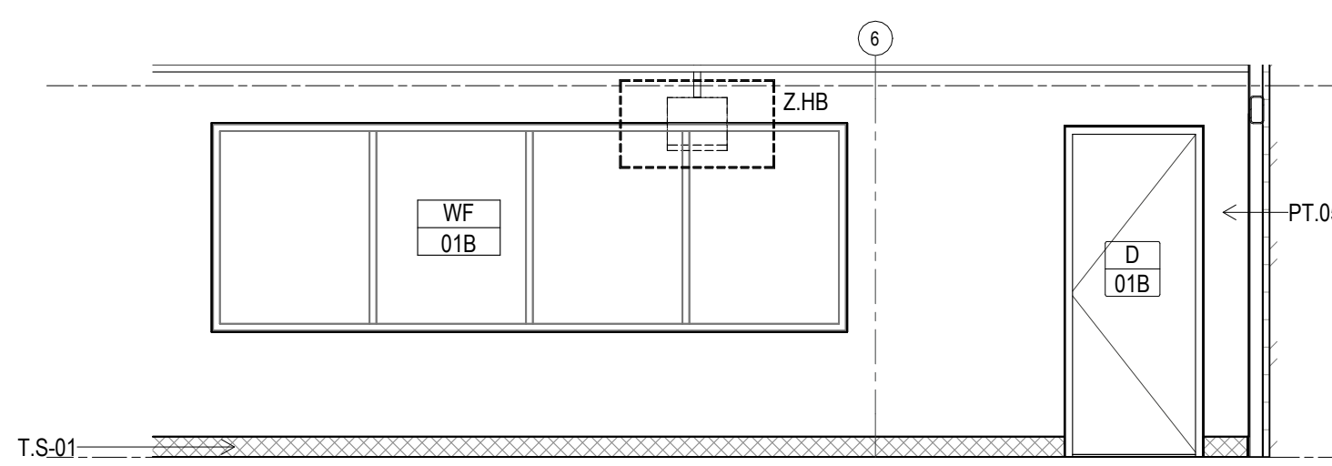
B ELEVATION MULTI-PURPOSE ROOM Scale: 1 : 50
