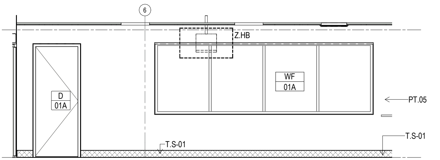
D ELEVATION MULTI-PURPOSE ROOM Scale: 1 : 50
