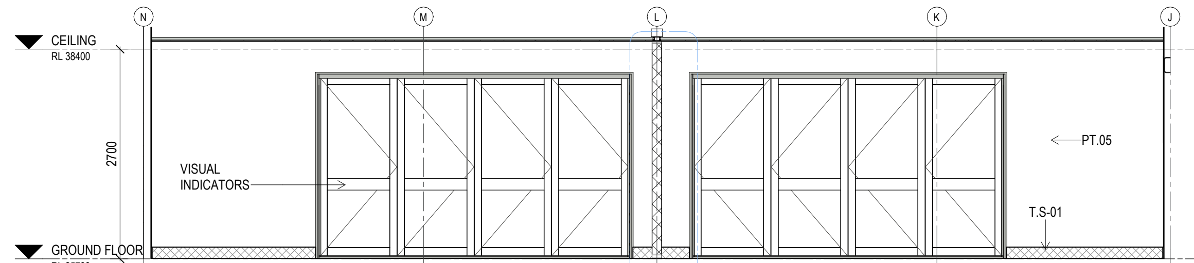
C ELEVATION MULTI-PURPOSE ROOM Scale: 1 : 50
