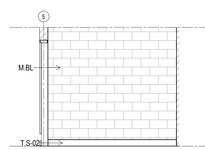
4 ELEVATION STORAGE Scale: 1 : 50
